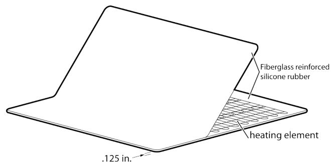
Heating Element Diagram
