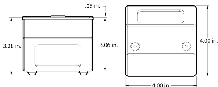
Camera Dimensions
