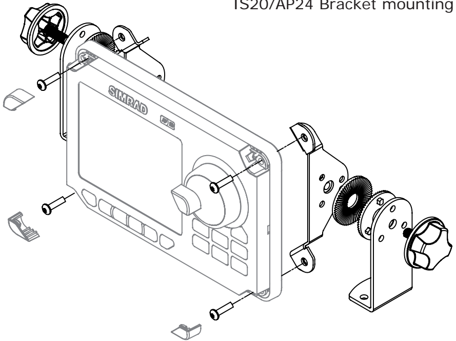
AP28 Bracket mounting
