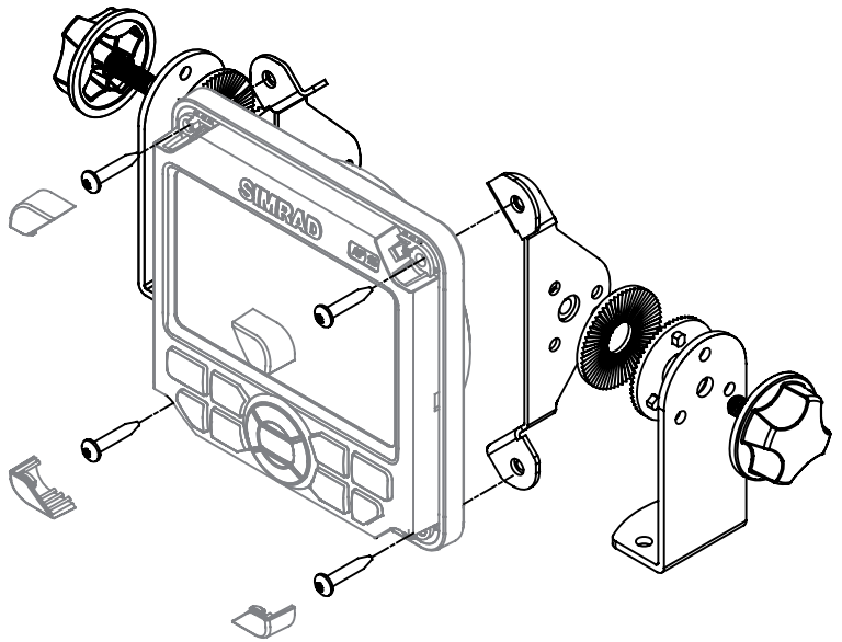
IS20/AP24 Bracket mounting
